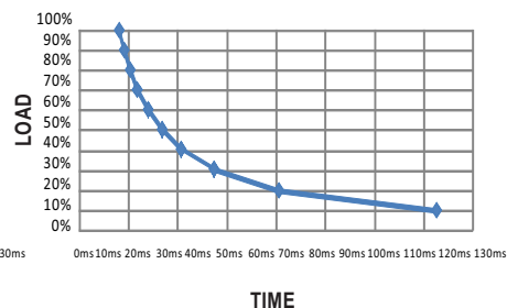
DDR-120D-48
